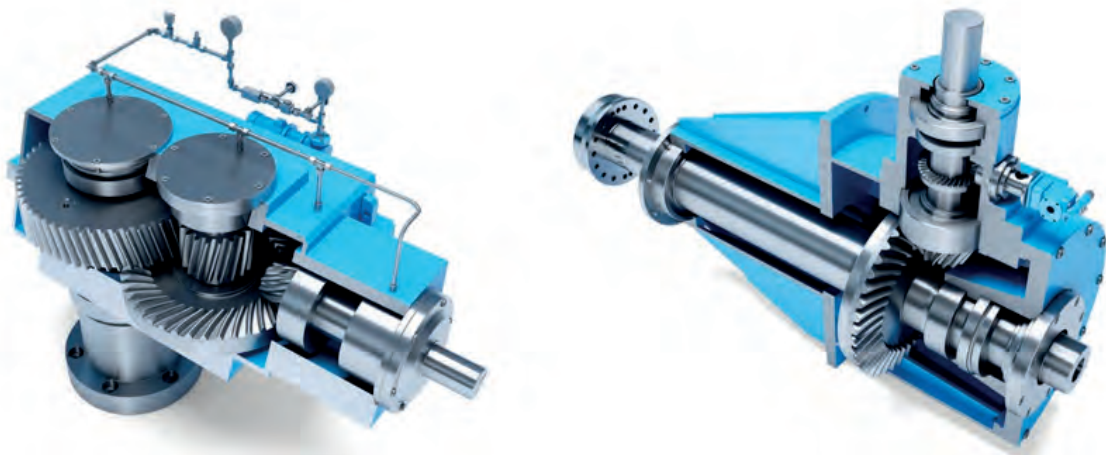
Figure 50: Bevel gears driving a horizontal (left) and vertical (right) generator (Eisenbeiss, 2016)
