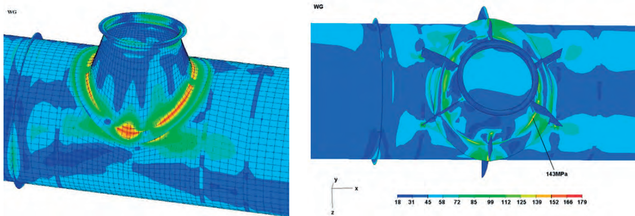
Figure 70: Tensile effort ( \text{MN/m}^2 ) distribution at penstock branching node (Adamkowski et al, 2019)
