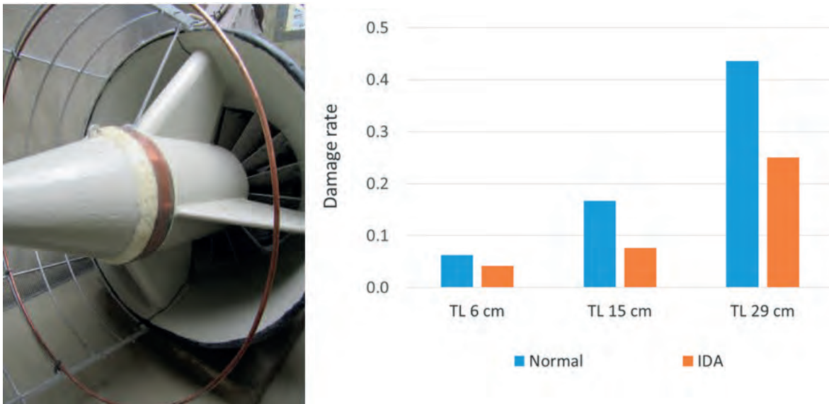
Figure 83: IDA pilot at the 35 kW test case Kaplan turbine intake with the two ring-shaped copper electrodes (left) and observed damage rates for fish passage without (blue) and with IDA pilot device (red) for varying fish lengths (total length TL)
