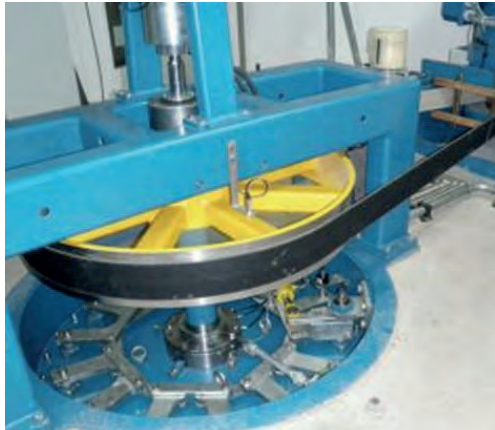
Figure 53: Flat belt drives in micro hydropower installations (Burger Wasserkraftanlagen, 2020)
