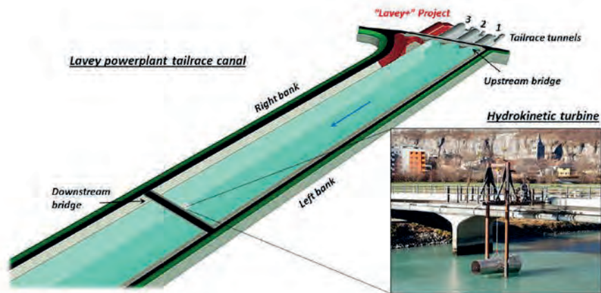
Figure 42: Tailrace channel of Lavey HPP with the open-air platform to test the kinetic turbine prototype (Munch et al., Water 2018)
