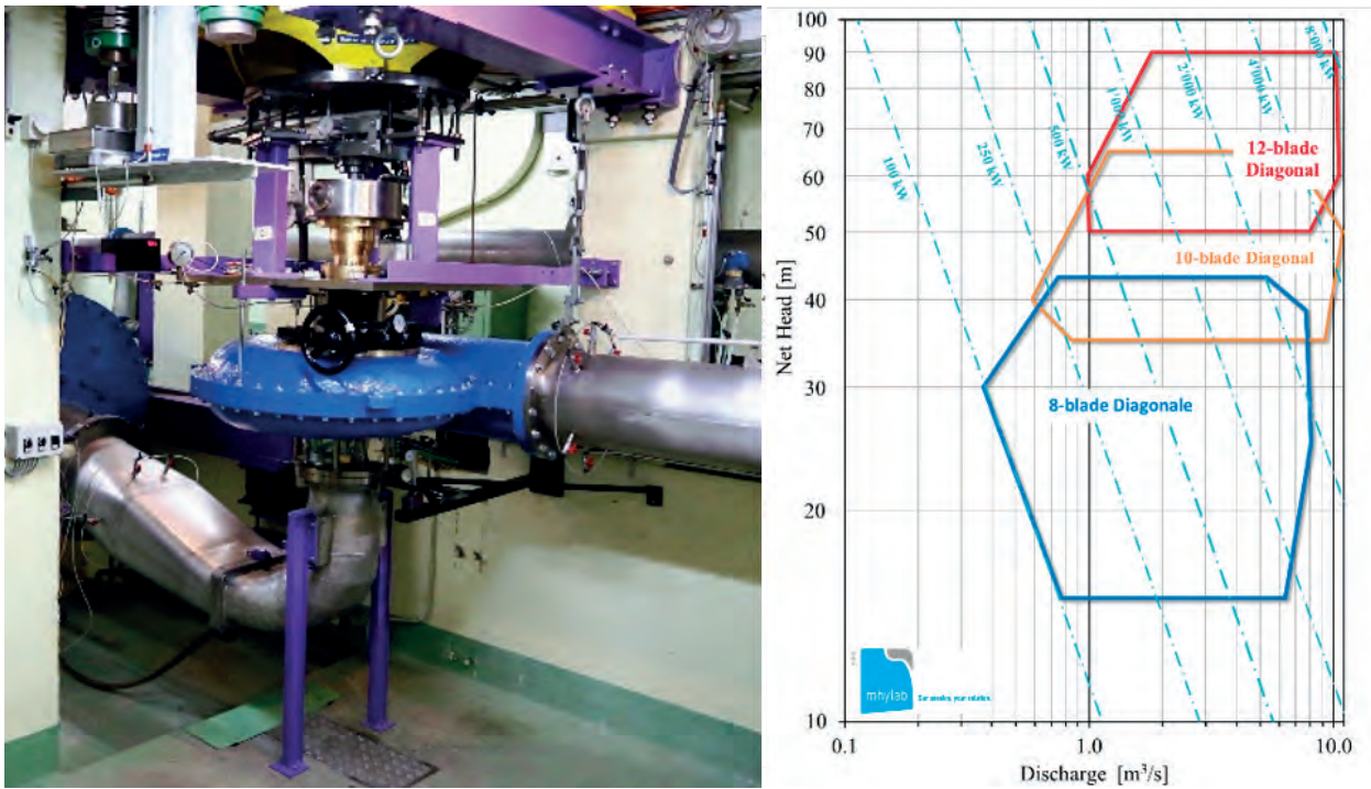
Figure 34: The Mhylab diagonal turbine (Bullani and Denis, 2019)
