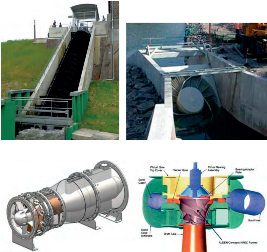
Figure 82: View of fish-friendly turbines: screw (up left), VLH (up right) (source: MJ2 technologies), Pentair fair-banks (down left) and Alden turbine (down right)
