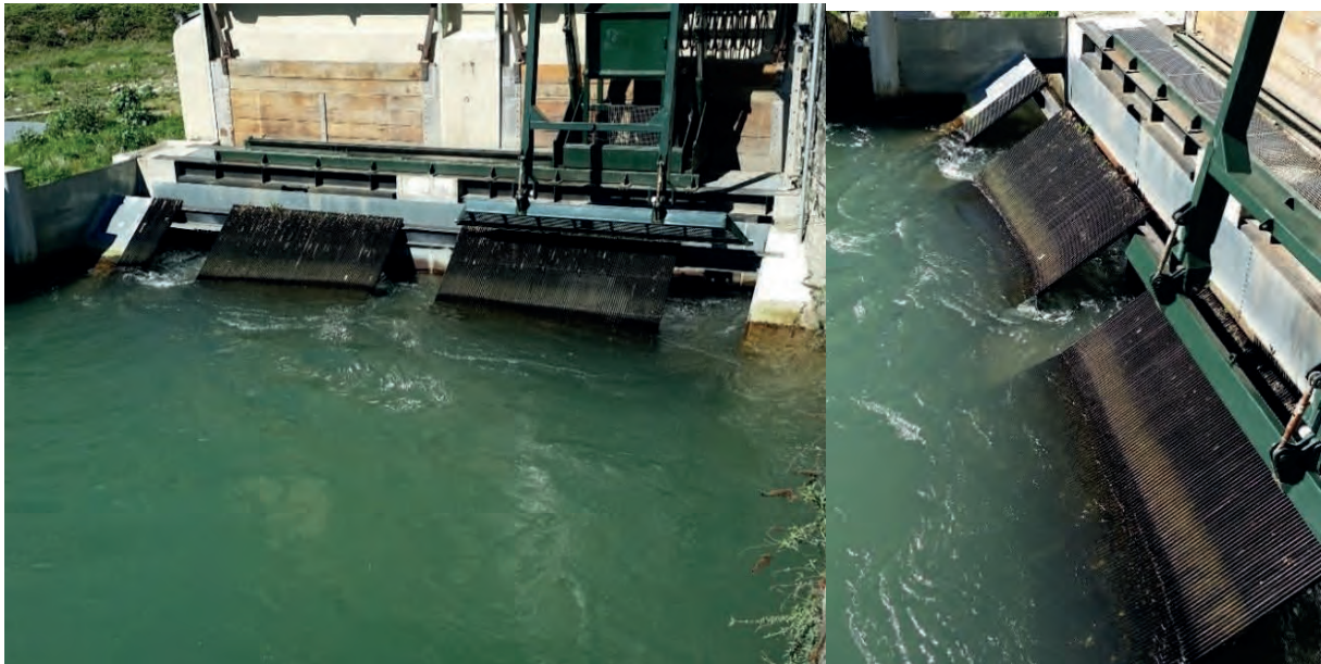
Figure 87: Inclined bar rack with openings to the bypass channel system (source: P. Rutschmann)
