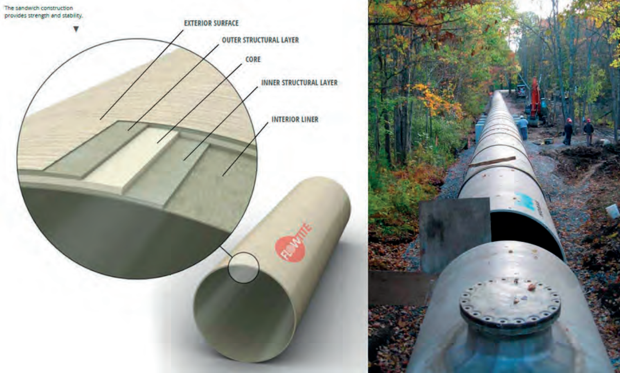
Figure 73: Flowtite pipe structure (left) and replacement of a wood stave penstock segment by a Hobas GRP pipeline (right). Jackman Hydro Station, Hills-borough, New Hampshire, USA (Amiblu, 2020)
