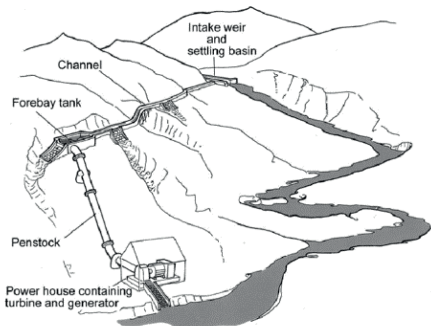
Figure 3: Schematic of a small hydro diversion scheme (Gatte and Kadhim, 2012)
