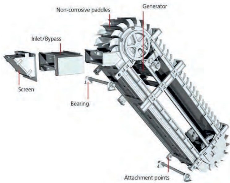
Figure 46: Steffturbine™ hydropower engine (Baselt, Malcherek and Maerker, 2013)
