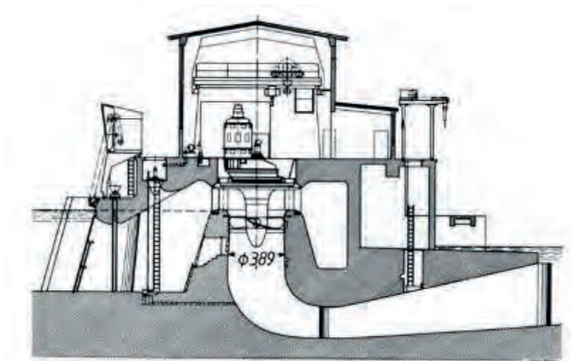
Figure 22: Classic Kaplan turbine in siphon configuration. Marktbreit SHP ( H = 2.5 m, P = 1100 kW) - Main, Germany (source: Raabe, 1985, after Voith)
