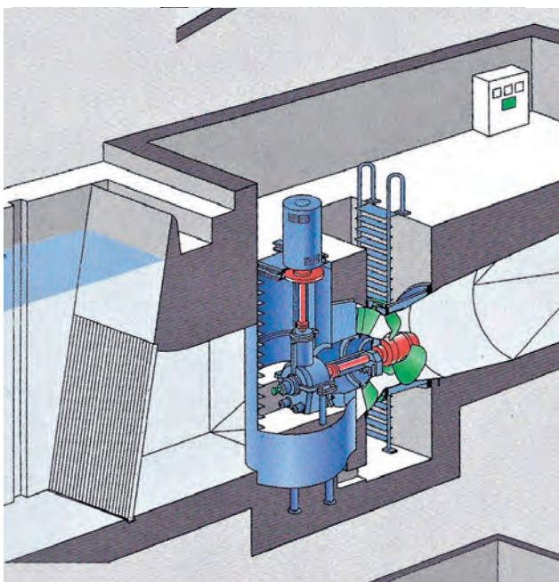
Figure 47: Tubular pit turbine with a bevel speed increaser (Voith, 1990s)
