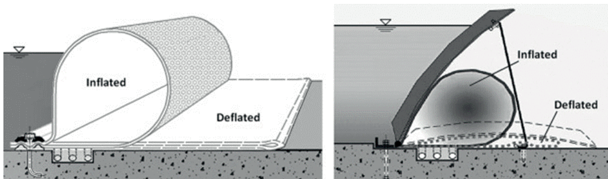
Figure 66: Inflated weir principle of operation (Daniel & Paulus, 2019)
