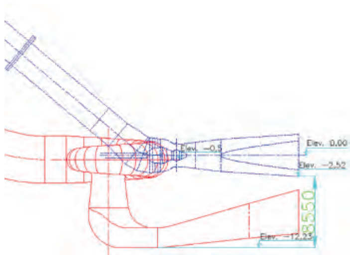
Figure 27: Comparison between excavation work needed for classic Kaplan turbines (2 units) and 4 tubular SAM turbines (4 units) with the same total capacity (Czerwinski, Canas, and Marin, 2012)
