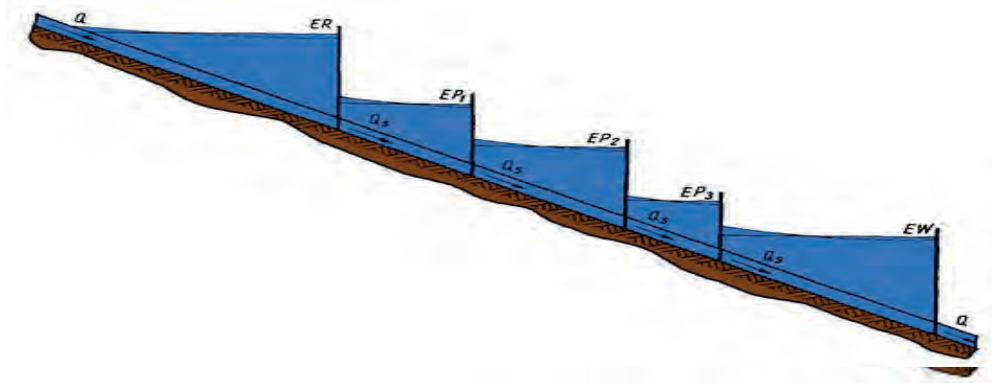
Figure 8: Schematic of a compact river cascade capable for swell operation without major water level variations at the intermediate stages (Michałowski and Plutecki, 1975)
